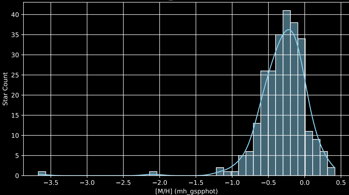
GALAH DR4 Field: [7132] [M/H] (mh_gspphot) (n= 258)
