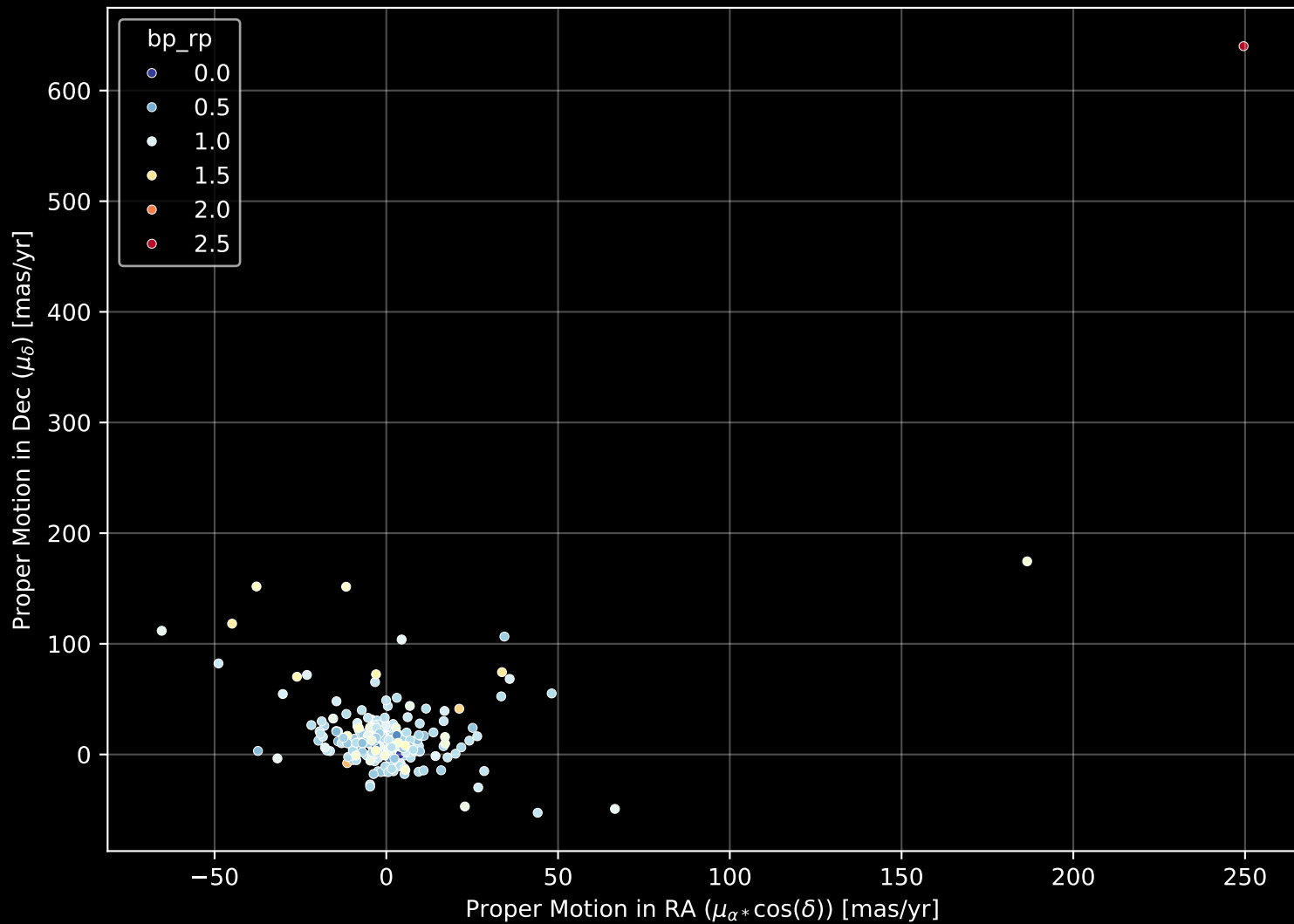
GALAH DR4 Field: [7132] Proper Motion Diagram (n= 259)
