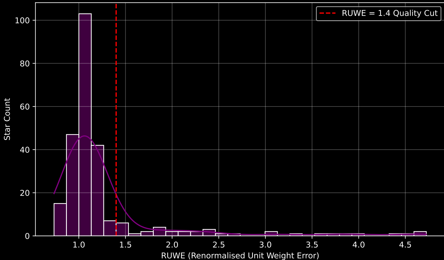
GALAH DR4 Field [7132] RUWE Distribution (n= 249)
