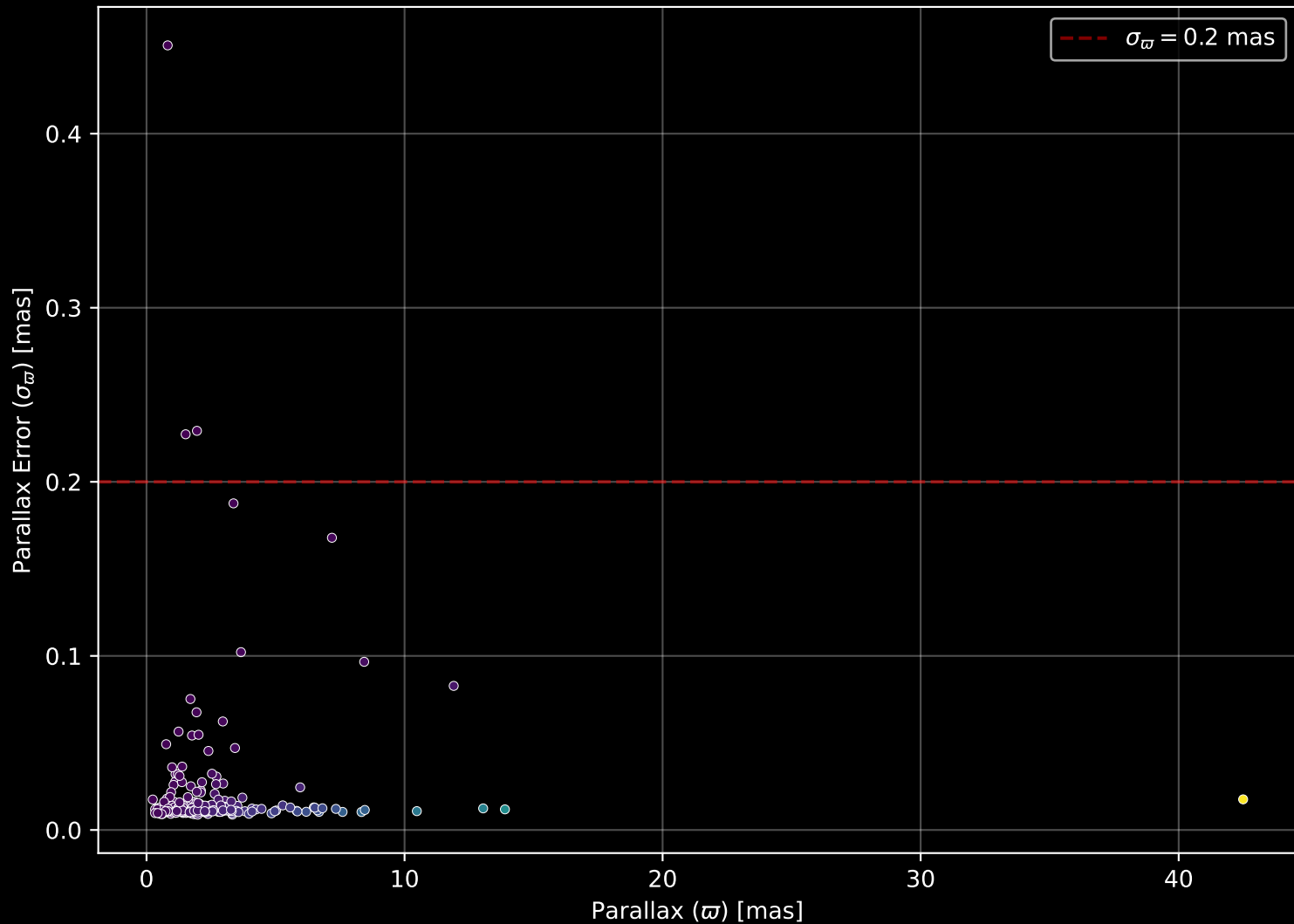
GALAH DR4 Field: [7132] Parallax Quality (n= 259)
