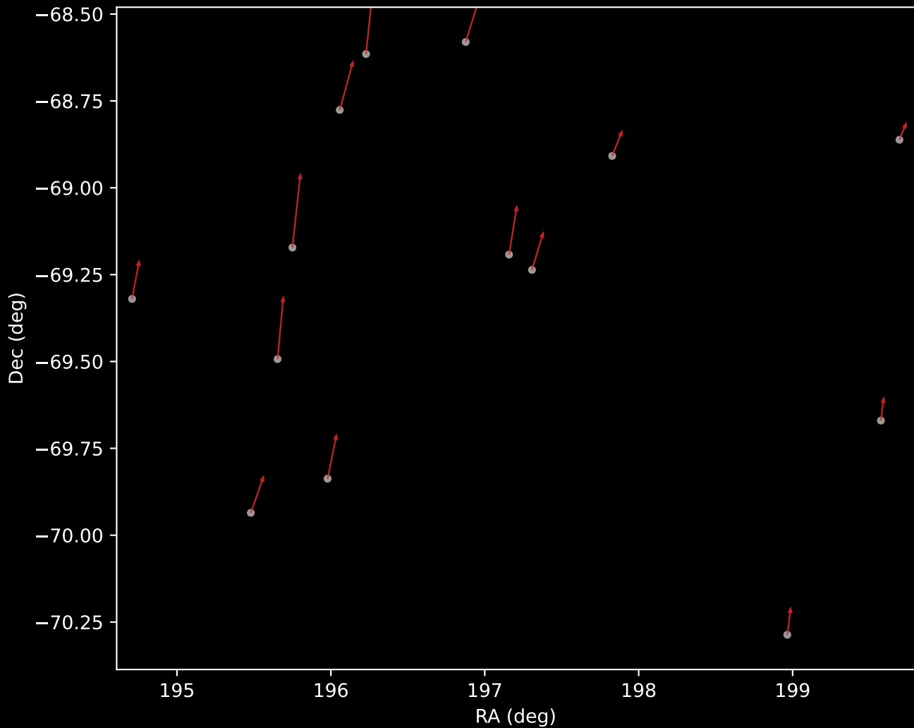
GALAH DR4 Cluster 6 Proper Motion Vectors (n=14)
