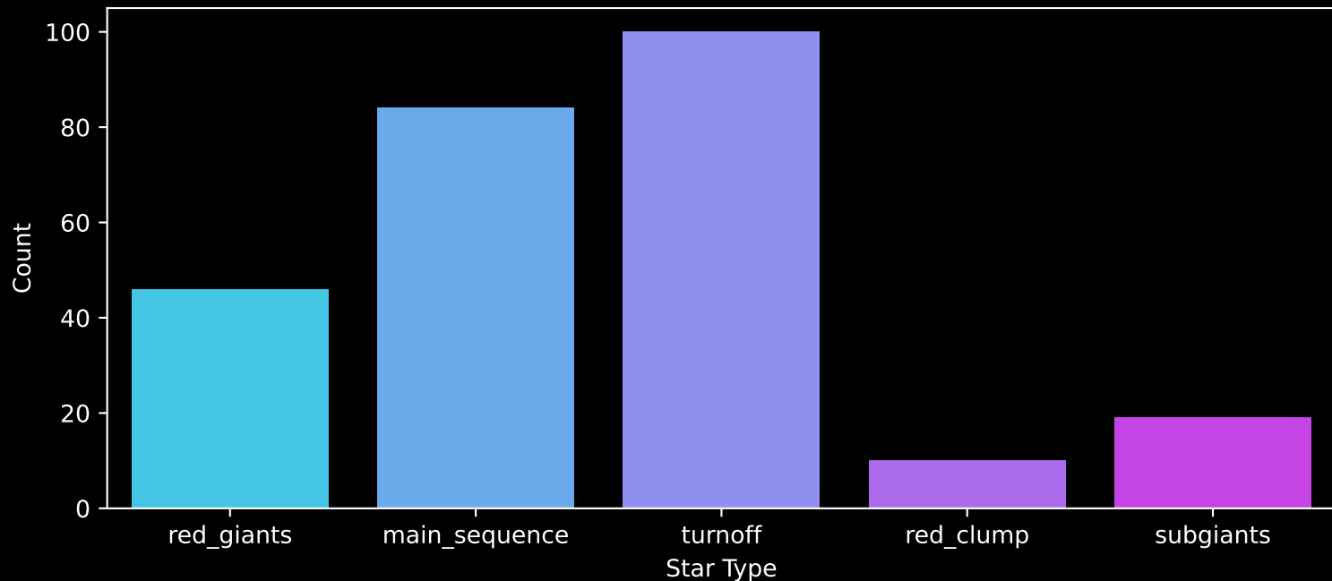
GALAH DR4 Field: [7132] Count plot of Star Type
